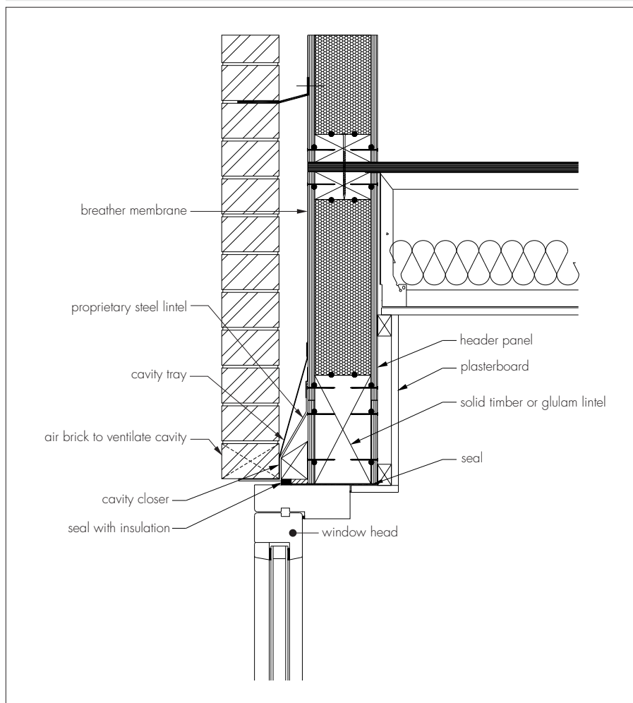
Figure 2 Typical lintel detail
