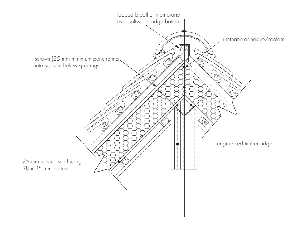
Figure 8 Typical roof detail at ridge
